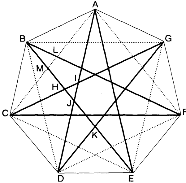
Figure 3. Seven-Pointed Star Forming Hexagon
